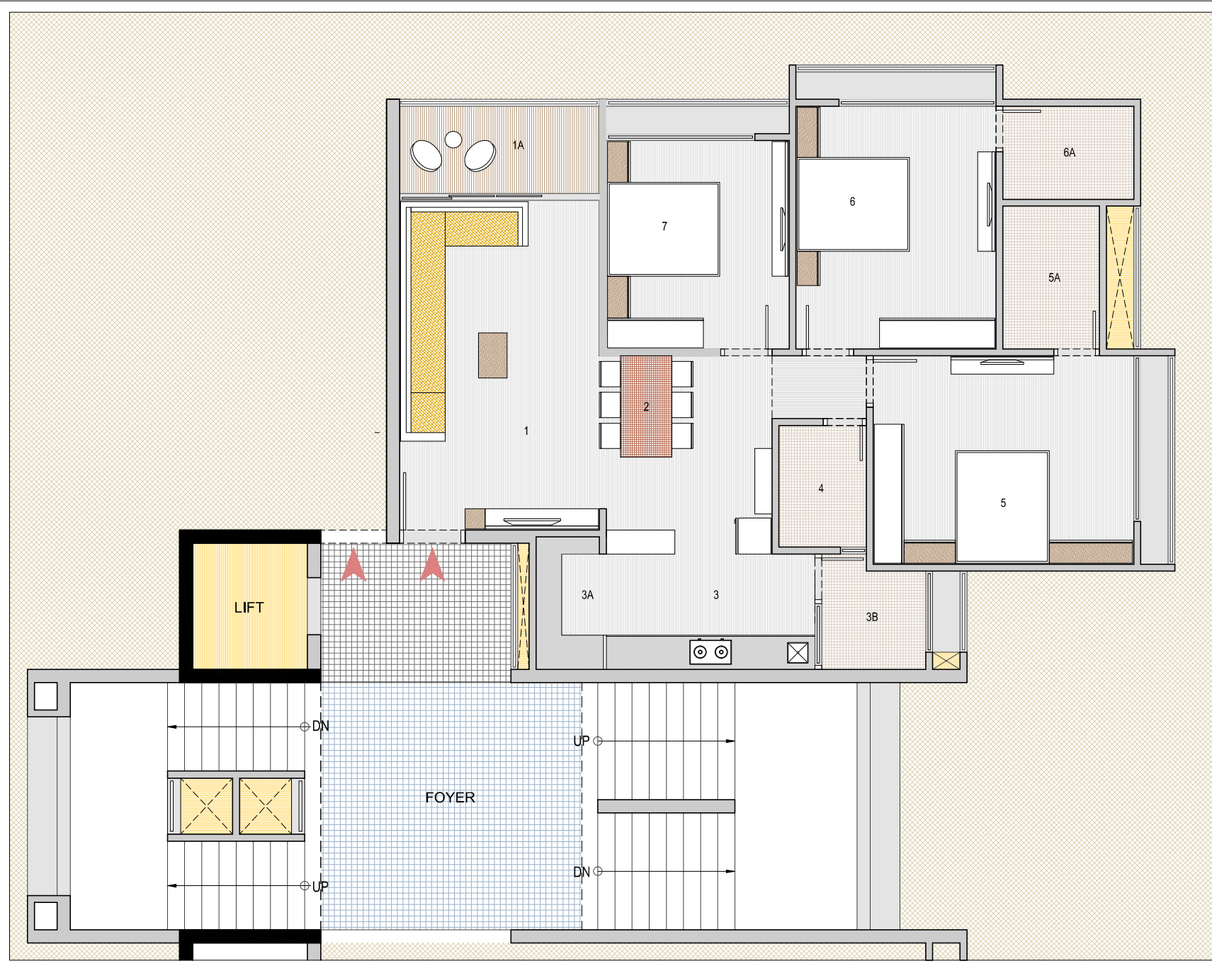
TYPICAL UNIT PLAN
