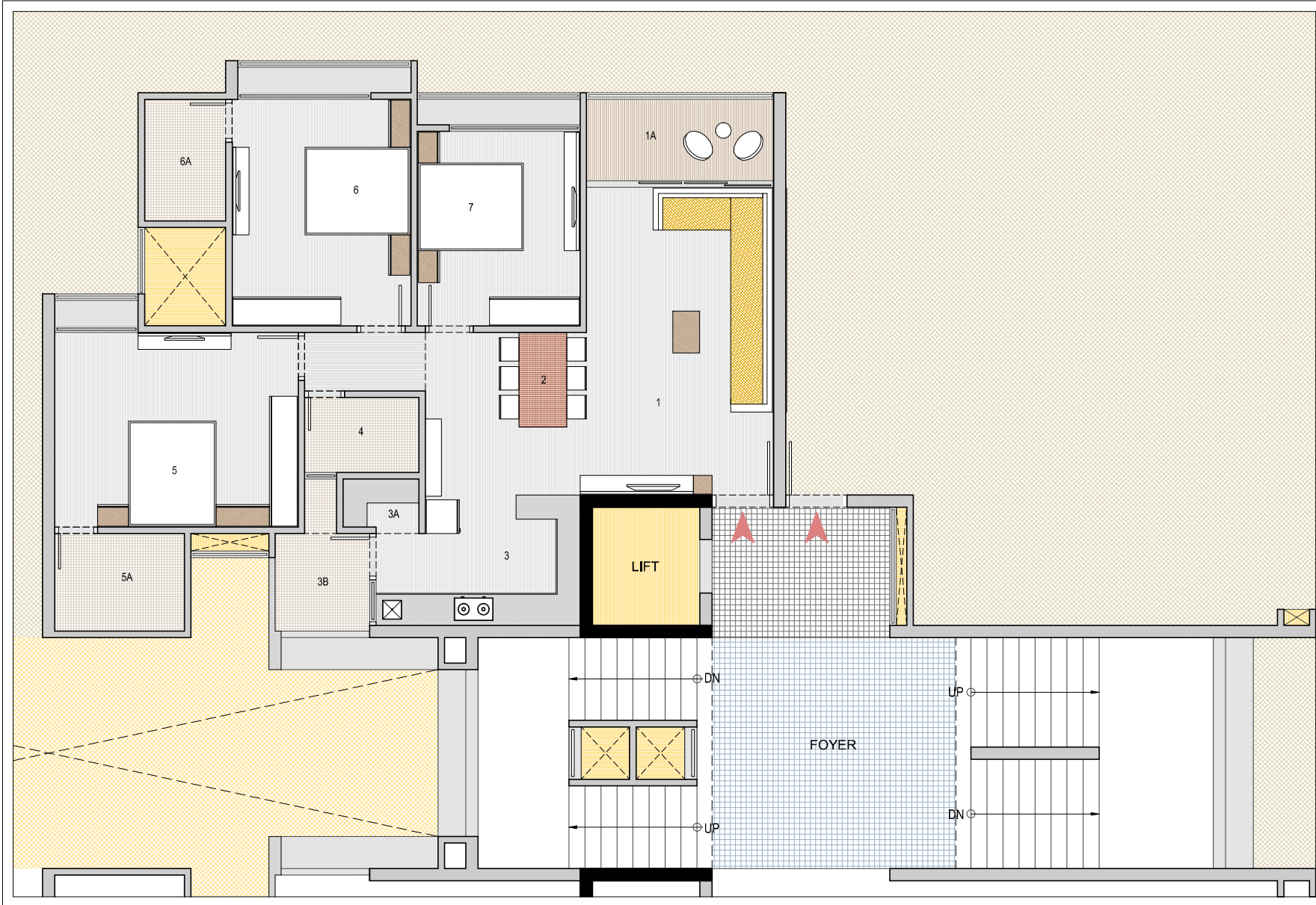
TYPICAL UNIT PLAN
